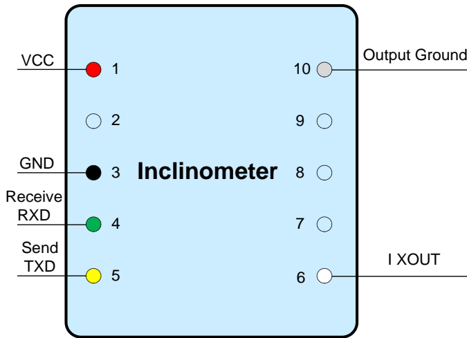
Figure 1. Pin Names
