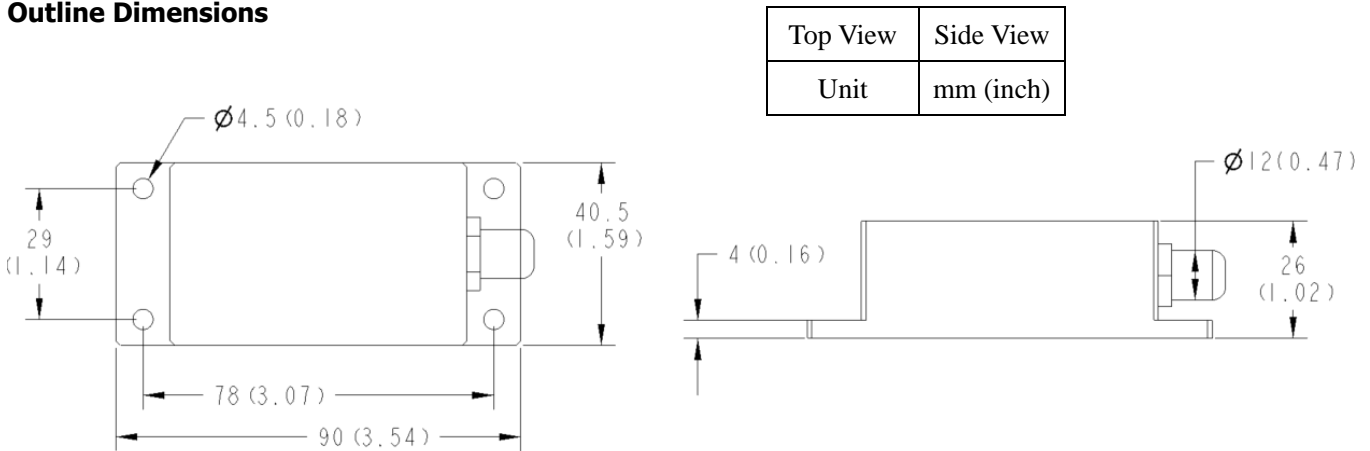
Figure 4. Outline Dimensions
