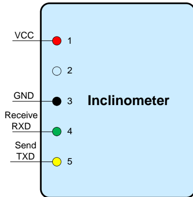
Figure 1. Pin Names
