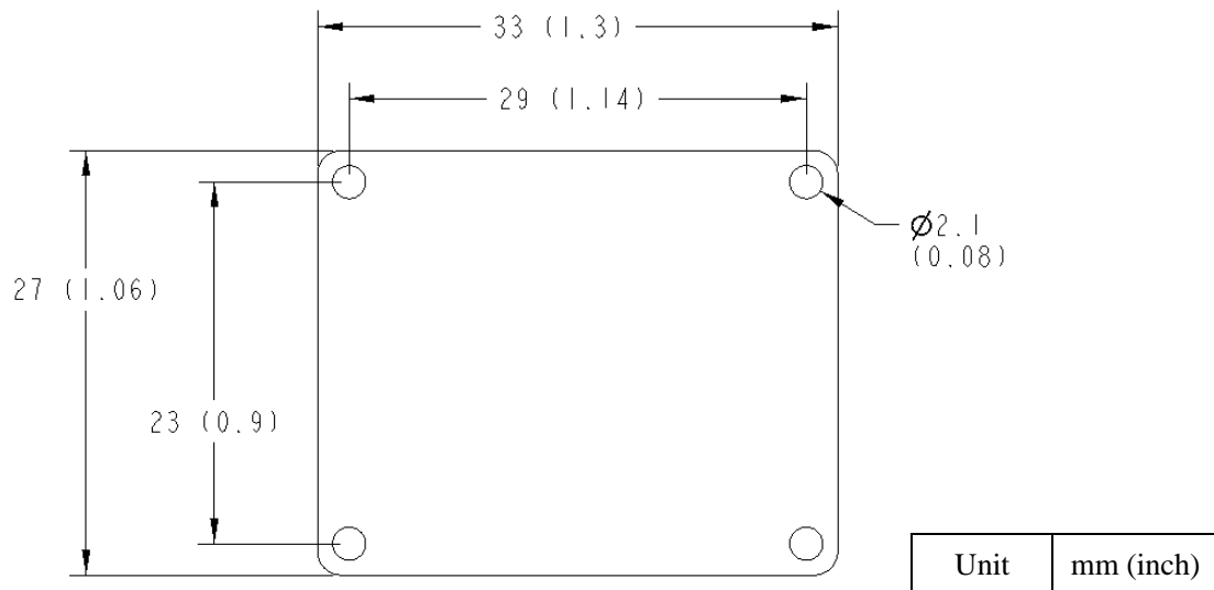
Figure 6. PCB Dimensions
