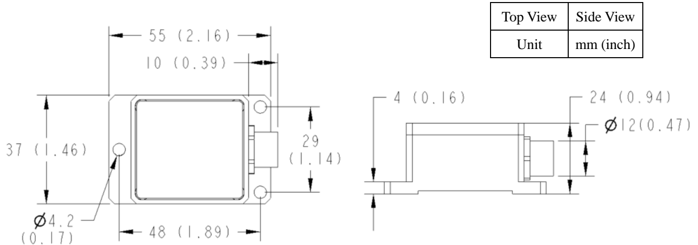
Figure 5. Outline Dimensions
