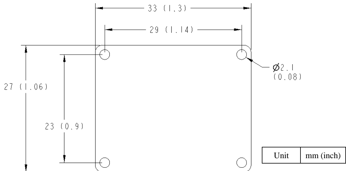
Figure 5. PCB Dimensions
