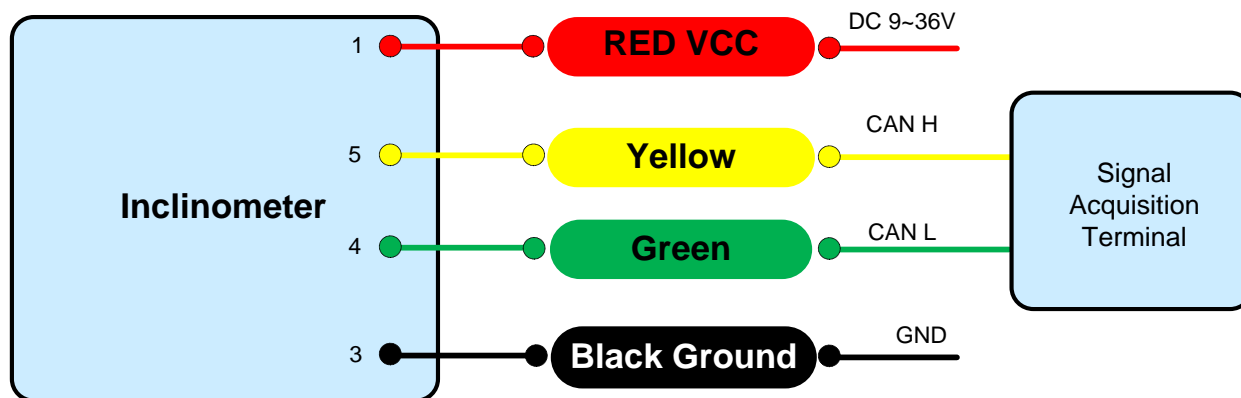
Figure 2. CAN Bus Wiring Diagram
