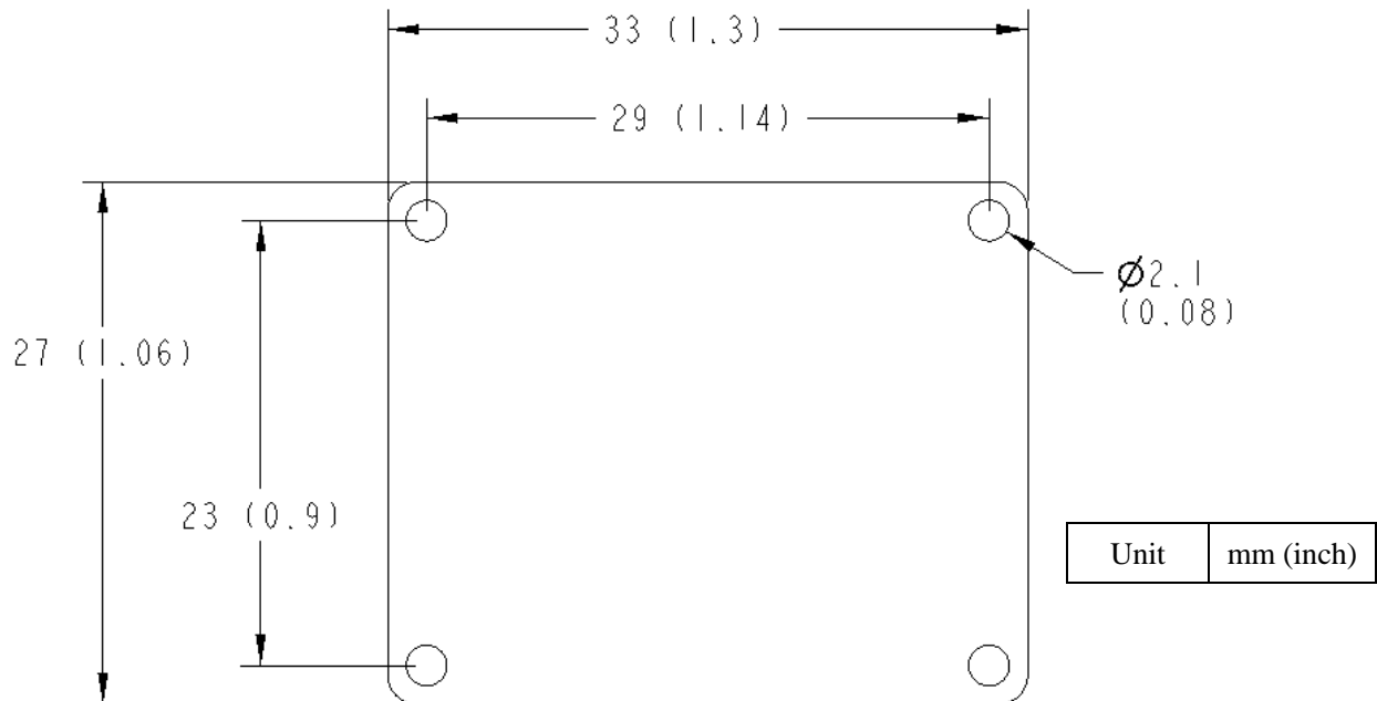
Figure 4. PCB Dimensions
