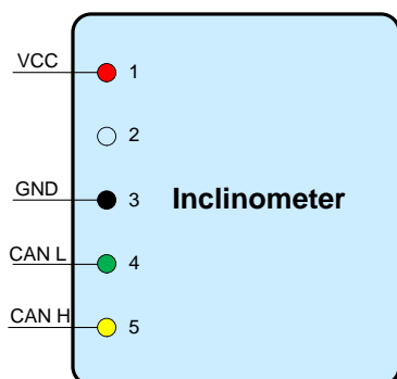
Figure 1. Pin Names
