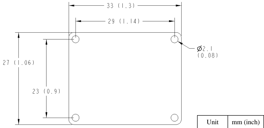
Figure 6. PCB Dimensions
