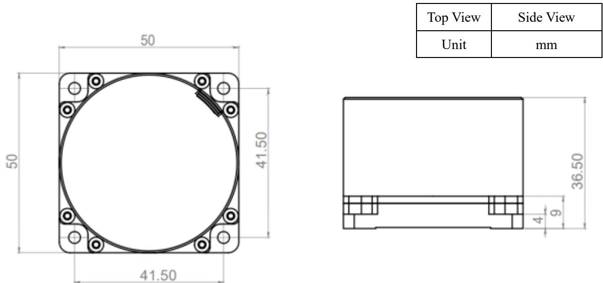
Figure 3. Outline Dimensions
