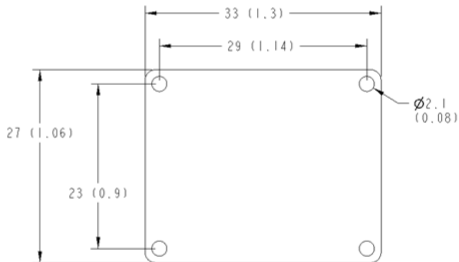
Figure 6. PCB Dimensions
