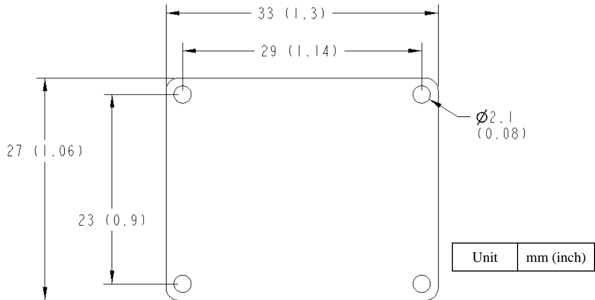
Figure 6. PCB Dimensions
