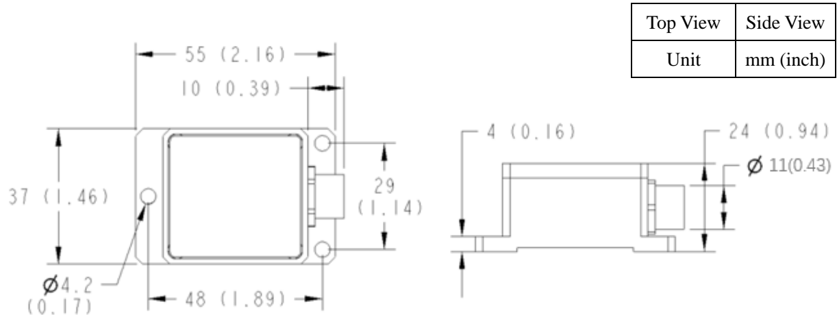
Figure 5. Outline Dimensions
