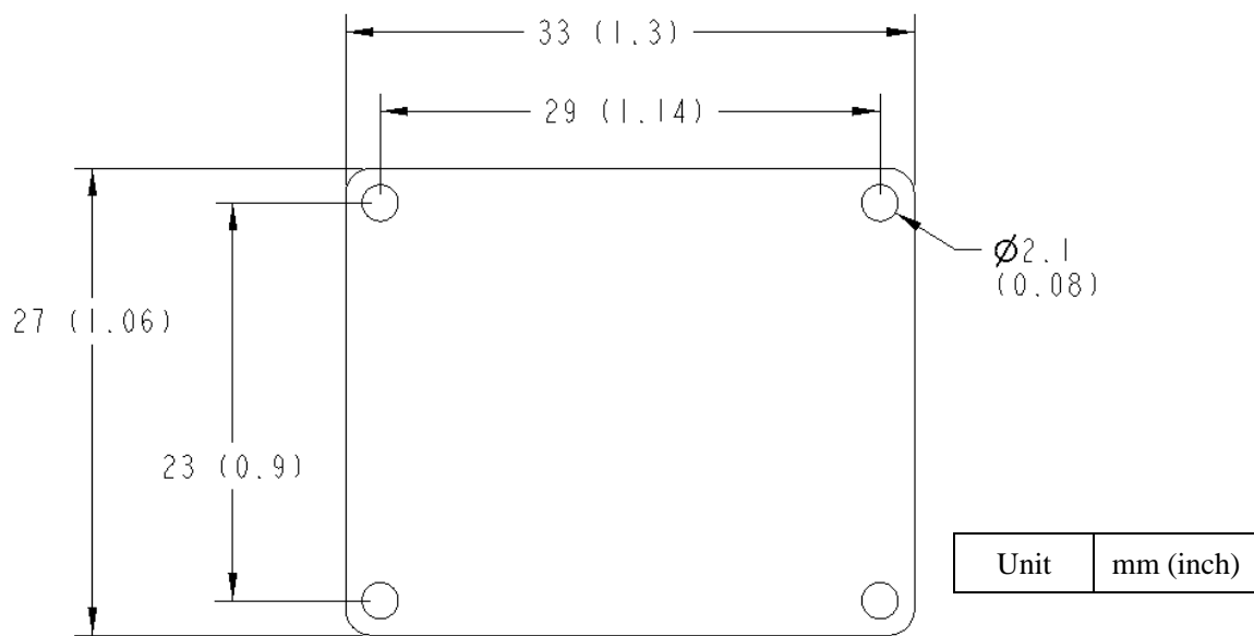
Figure 6. PCB Dimensions
