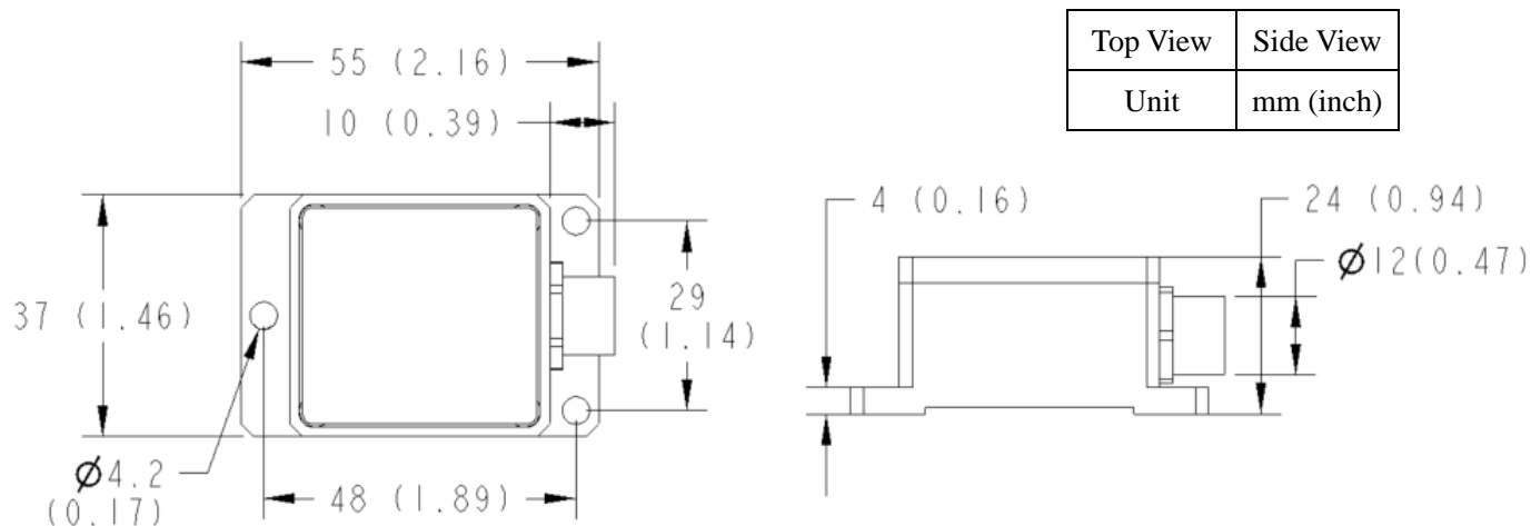
Figure 5. Outline Dimensions
