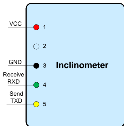
Figure 1. Pin Names
