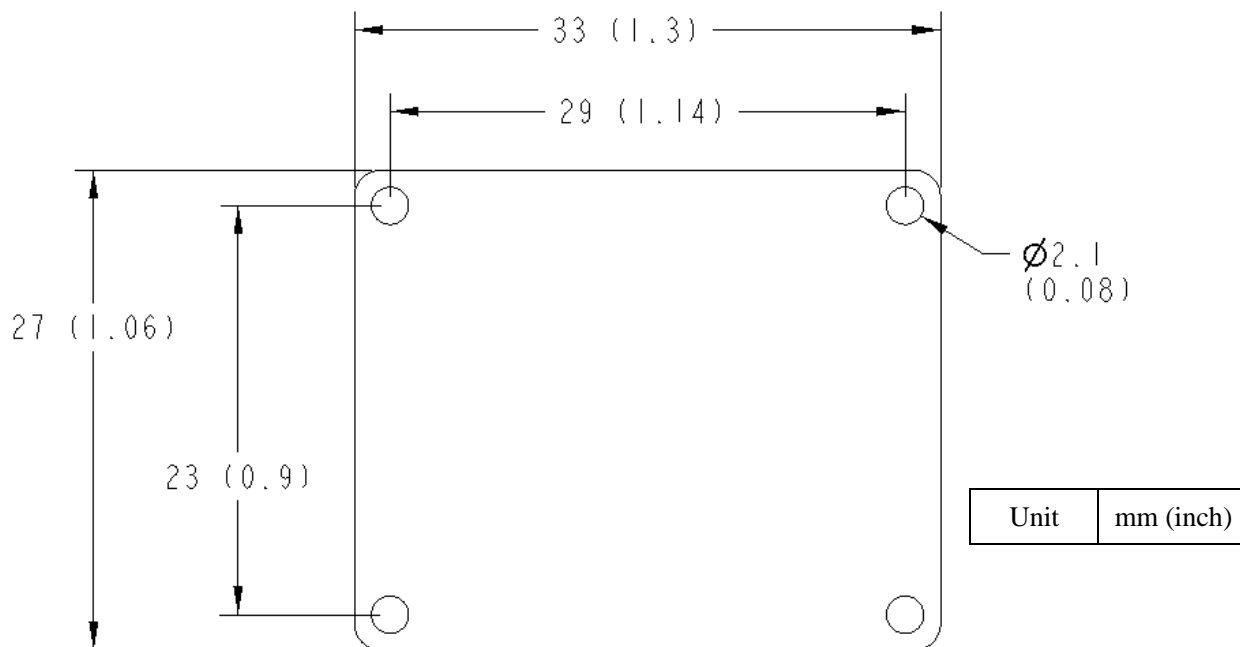
Figure 6. PCB Dimensions
