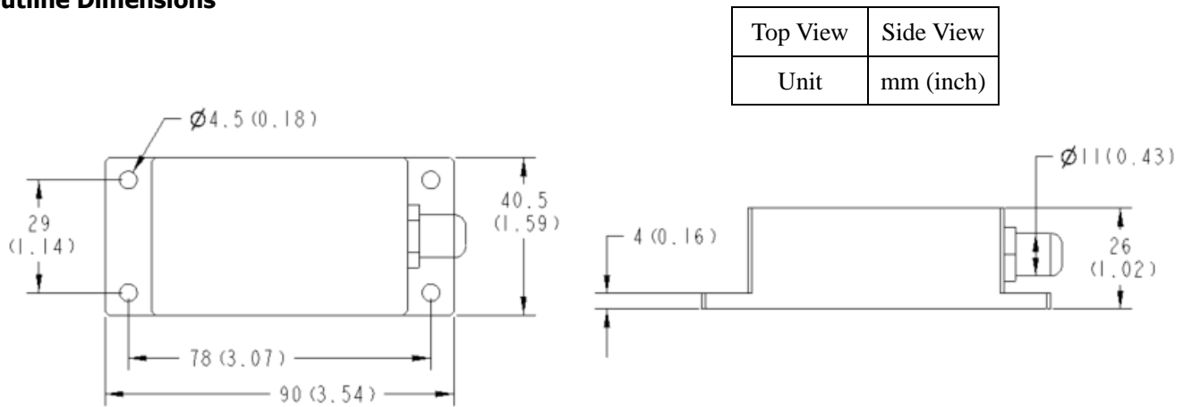
Figure 4. Outline Dimensions
