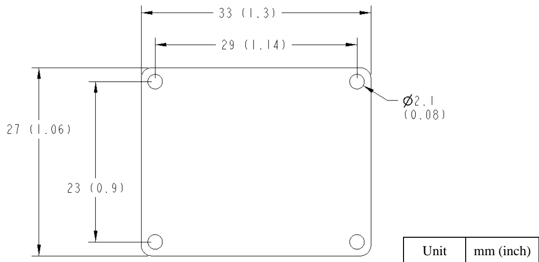
Figure 6. PCB Dimensions
