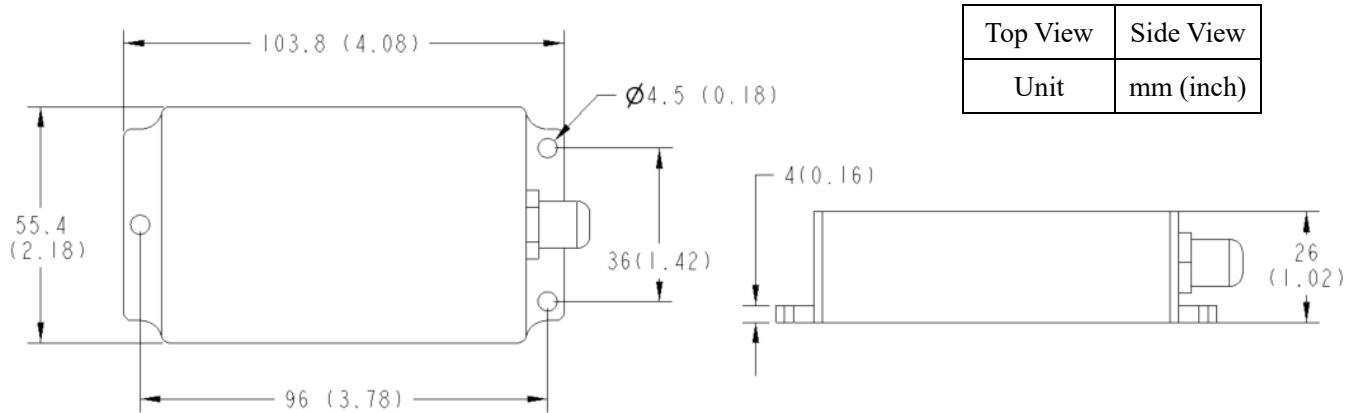
Figure 4. Outline Dimensions
