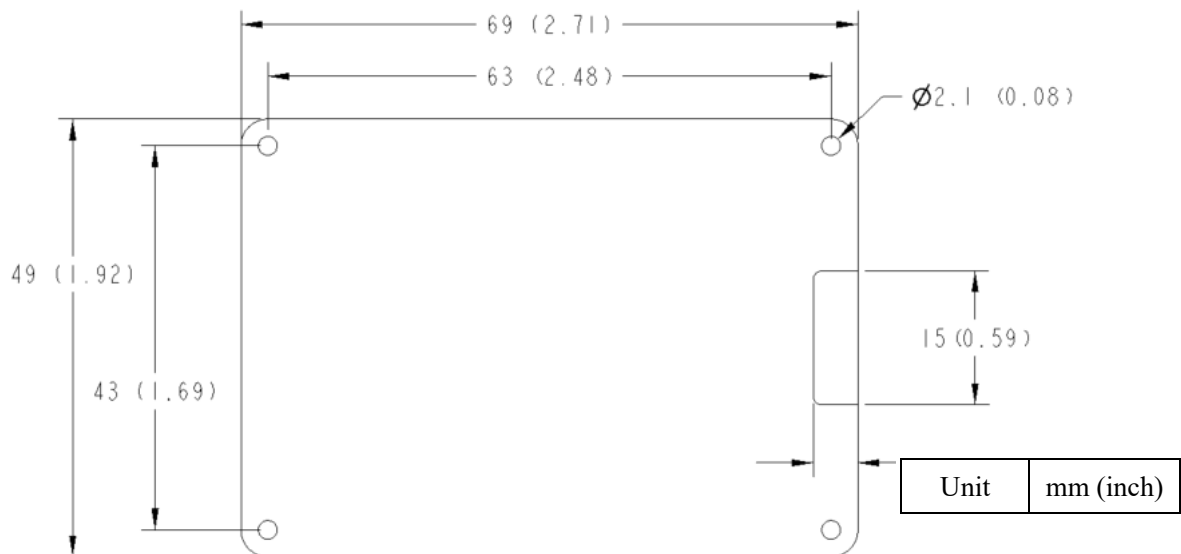
Figure 5. PCB Dimensions
