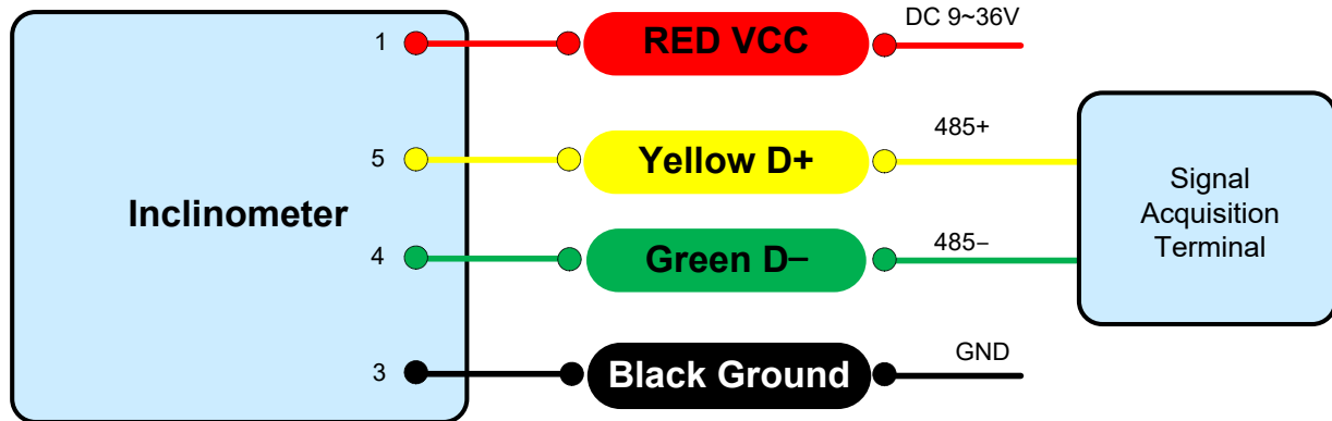
Figure 1. RS 485 Wiring Diagram
