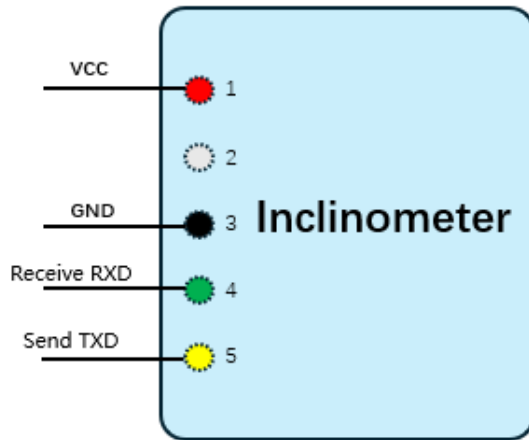
Figure 1. Pin Names
