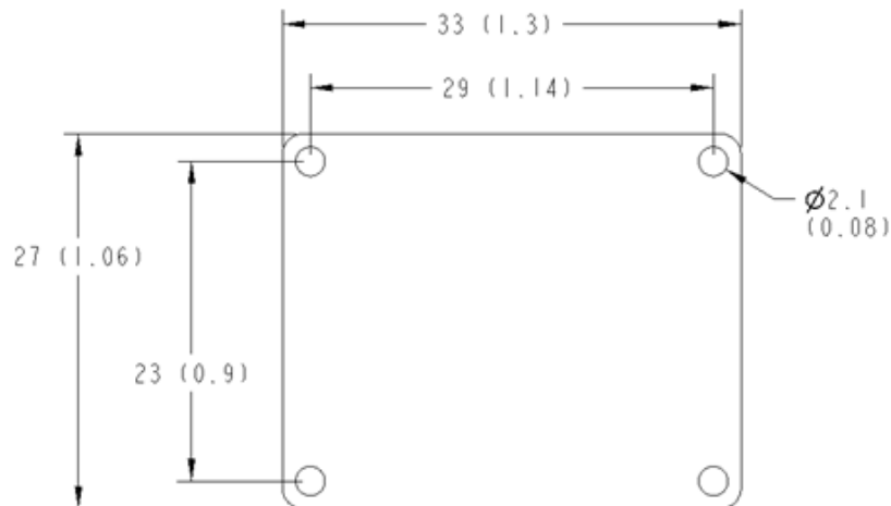
Figure 4. PCB Dimensions
