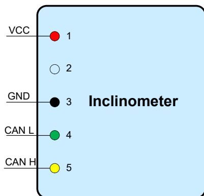
Figure 1. Pin Names
