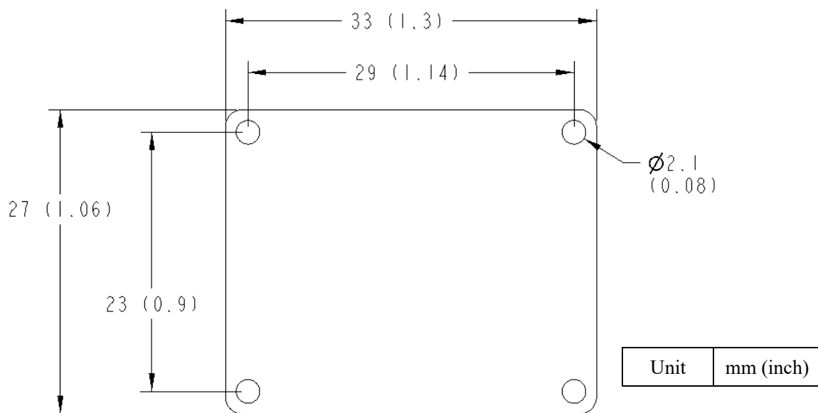
Figure 6. PCB Dimensions
