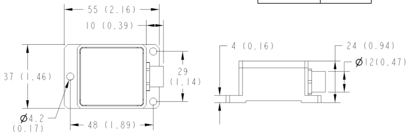
Figure 4. Outline Dimensions
